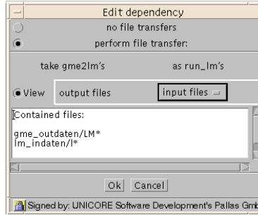
Figure 7: Dependency Definition
