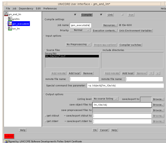
Figure 8: GUI for COMPILE Task
