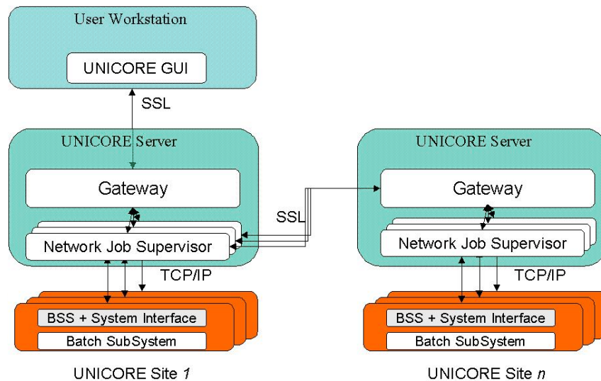
Figure 1: Architecture Overview
