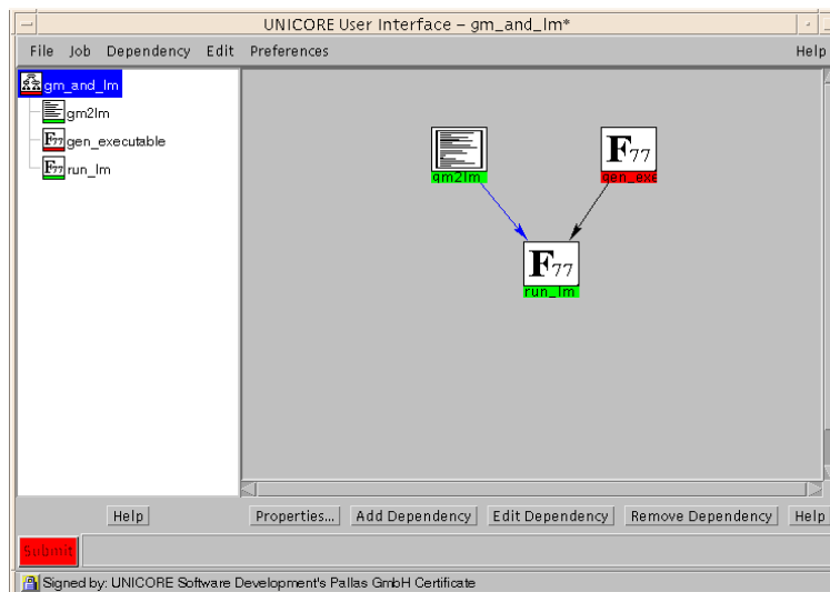
Figure 6: A Job Example
