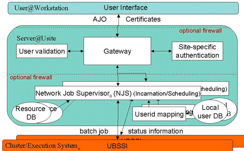
Figure 3: The UNICORE Server Tier
