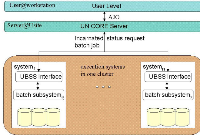
Figure 4: The Target System Tier
