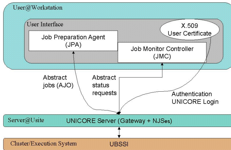
Figure 2: The User Tier
