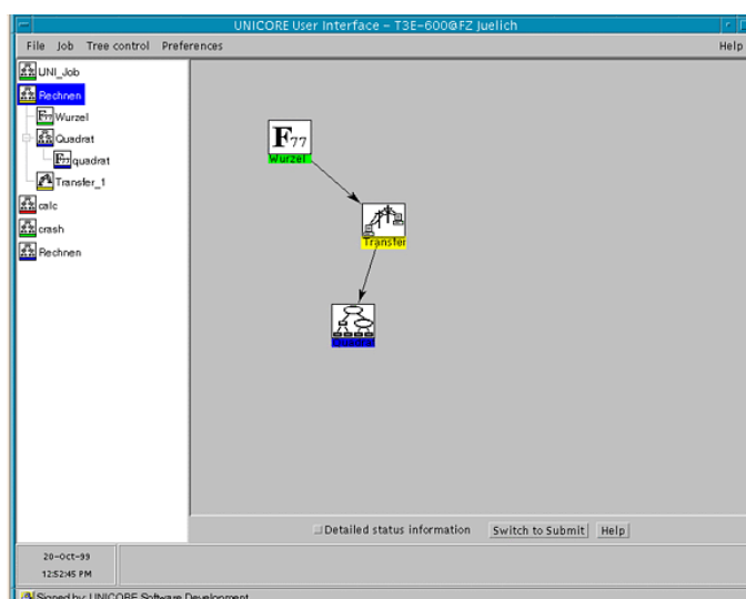
Figure 10: Job Monitor Controller
