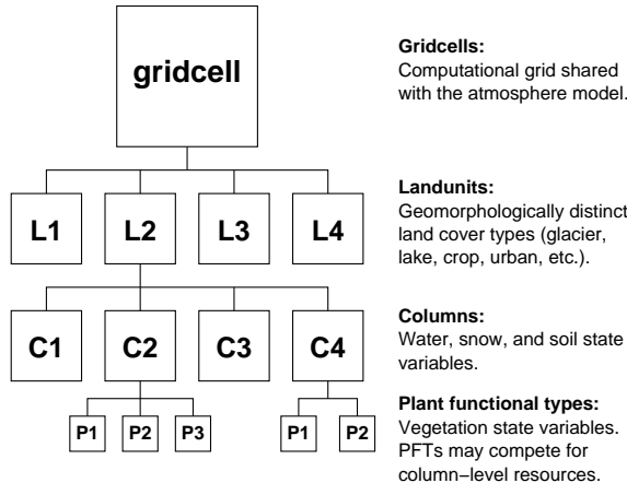
Figure 1: The CLM subgrid hierarchy
