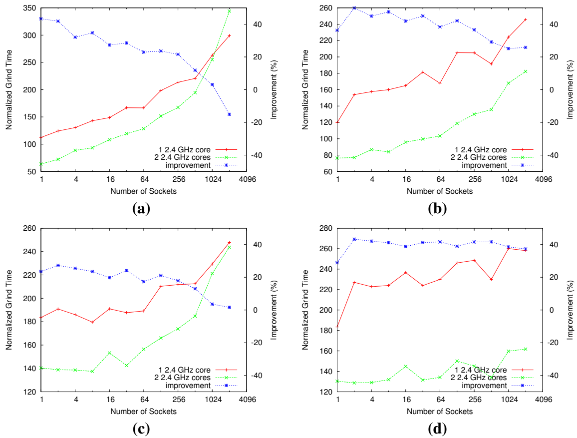
Fig. 6. Percent improvement for PARTISN diffusion (a, c) and transport (b, d) portions for 24^3 (a, b) and 48^3 (c, d) problems
