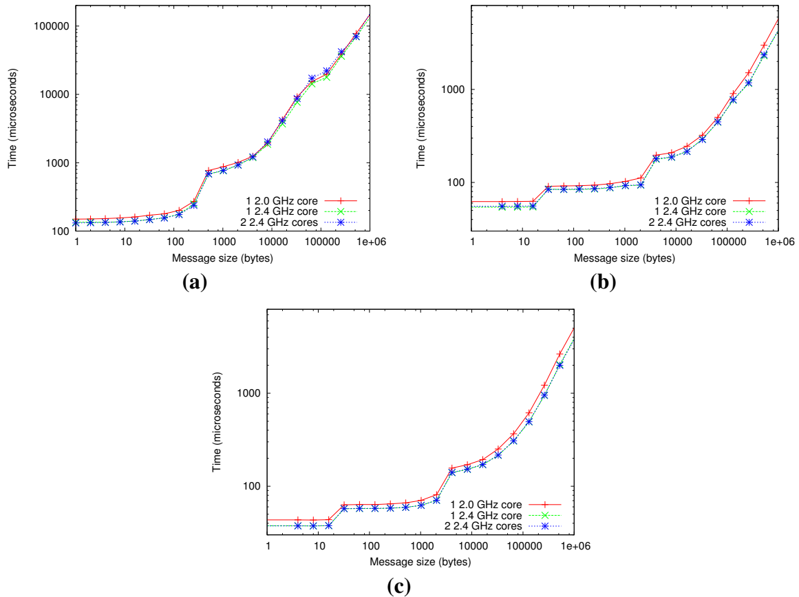
Fig. 2. 64 node Pallas benchmarks for (a) Alltoall, (b) Allreduce, and (c) Reduce
