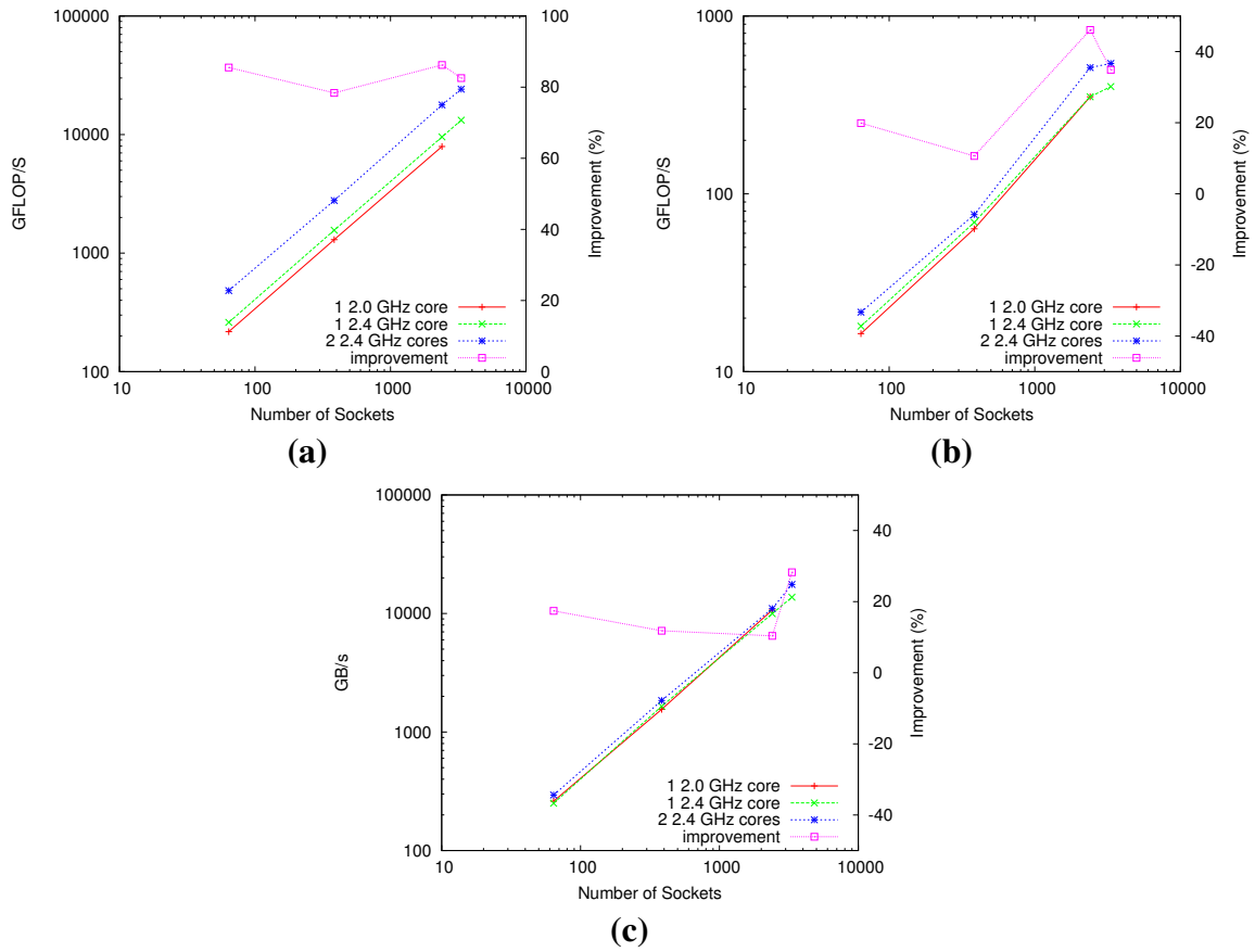
Fig. 3. (a) HPL, (b) FFT, and (c) STREAMS results
