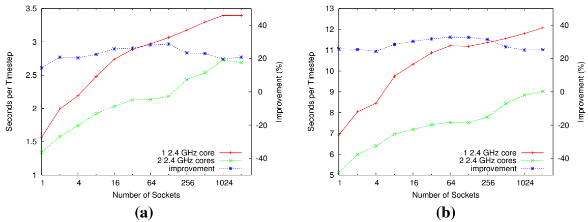
Fig. 7. Percent improvement for CTH sizes 50x120x50 (a) and 80x192x80 (b)
