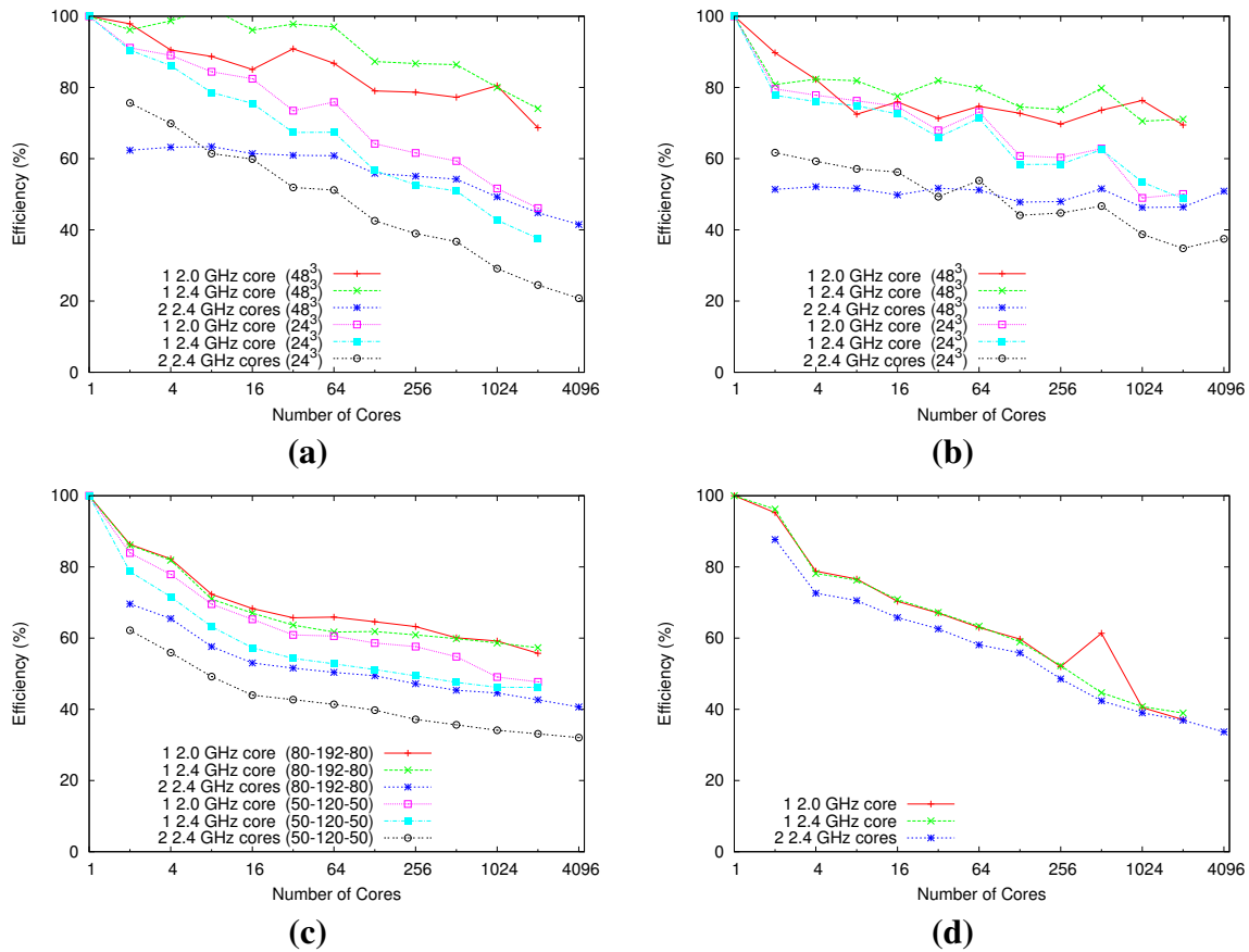
Fig. 5. Parallel efficiency impacts on PARTISN (a) diffusion and (b) transport portions and parallel efficiency impacts on (c) CTH and (d) SAGE
