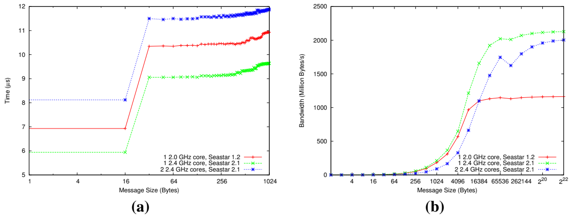
Fig. 1. Ping-pong latency (a) and streaming bandwidth (b)
