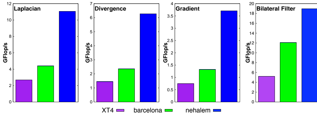
Figure 6. Performance summary. For the bilateral filter kernel, the chart shows average performance across the two radius values.
