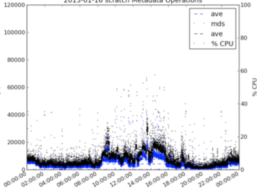
2013-01-16 scratch Metadata Operations
