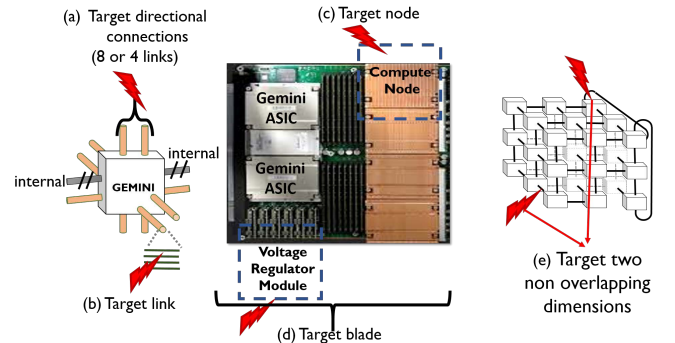
Fig. 1: Target components of fault injection experiments. A failure of a blade leads to failure of two ASICs.
