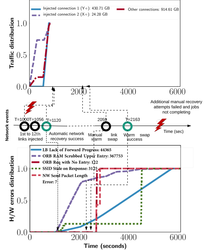
Fig. 8: Double connection injection and deadlock. Top : Cumulative distribution of network traffic measured in the time interval of the experiment. After the injection, the failure stalled the LDMS. Middle : Time series of network events (enlarged). Bottom : cumulative distribution of anomalous hardware error logs during the experiment.
