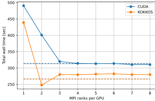
Fig. 3. Time to simulate 100 thousand diffraction patterns using 64 Perlmutter nodes. In contrast to Fig. 2, this benchmark includes the time to save each image to the file system. For comparison, the previous times without file saving are indicated with dashed lines. As the filesystem performance on Perlmutter can vary (due to it not being a production system) at the time of writing, this graph shows the best performance over several repeated runs.
