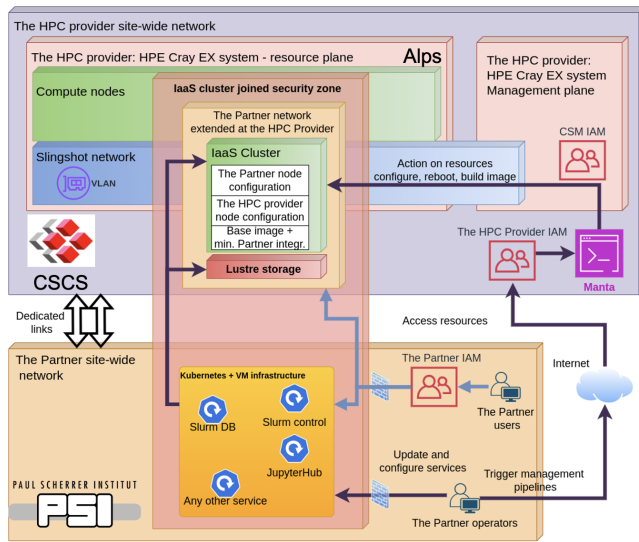
Figure 4: Tenant operational view, the IaaS cluster belongs to a jointly security zone and is integrated into PSI network. Operators can configure their services with existing mechanisms whereas they use an identity provided by CSCS to execute system management actions through Manta. For PSI's users access to the IaaS cluster is transparent.
